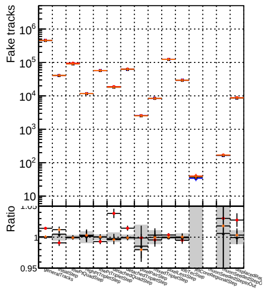
Number Legend 1 DQM_inklr_it_step2_ttbar-phase1-newgeom 2 DQM_angle_step2_ttbar-phase1-newgeom 3 DQM_fast_step2_ttbar-phase1-newgeom
