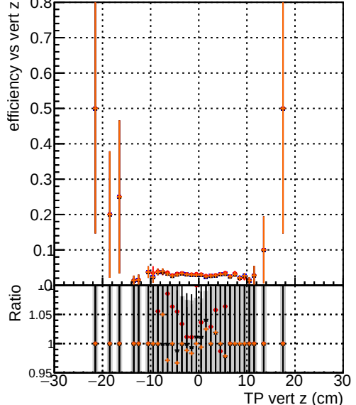
Efficiency vs. TP vert z (cm) Legend: - DQM_original_step2_ttbar-phase1-newgeom (blue line with circles) - DQM_mkFit_step2_ttbar-phase1-newgeom (red line with crosses) - DQM_angle_step2_ttbar-phase1-newgeom (black line with crosses) - DQM_fast_step2_ttbar-phase1-newgeom (orange line with crosses)
