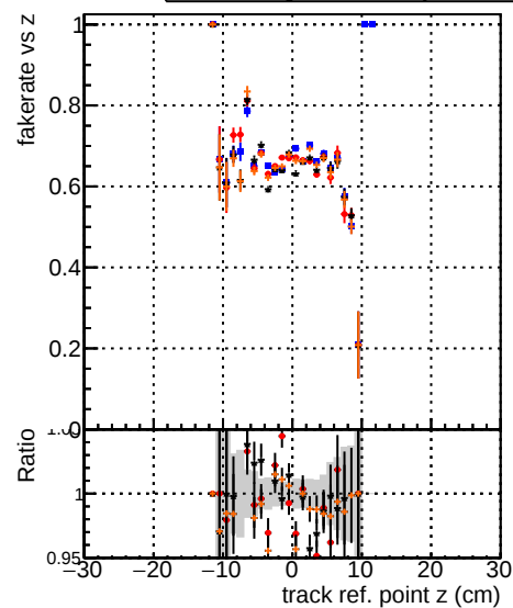
DOM original_step2_ttbart-phase1-newgeom DOM mkr-it_step2_ttbart-phase1-newgeom DOM angle_step2_ttbart-phase1-newgeom DOM fast_step2_ttbart-phase1-newgeom
