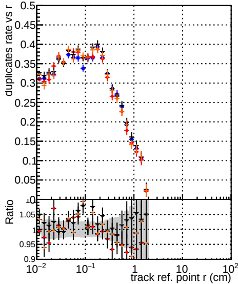
DOM original_step2_ttbart-phase1-newgeom DOM mkr-it_step2_ttbart-phase1-newgeom DOM angle_step2_ttbart-phase1-newgeom DOM fast_step2_ttbart-phase1-newgeom
