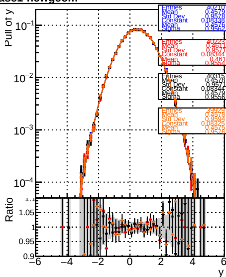
Legend for Pull of y for PV: DOM original_step2_ttbbar-phase1-newgeom DOM mkfit_step2_ttbbar-phase1-newgeom DOM angle_step2_ttbbar-phase1-newgeom DOM fast_step2_ttbbar-phase1-newgeom
