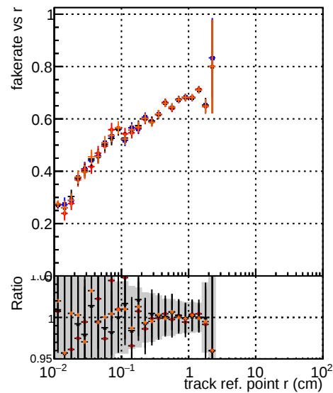
Legend for Fake rate vs verpos, Duplicates Rate vs verpos, and Pileup rate vs verpos: DOM original (blue circles) DOM step2 (red circles) DOM t1bar-phase1 (black circles) DOM newgeom (orange circles)
