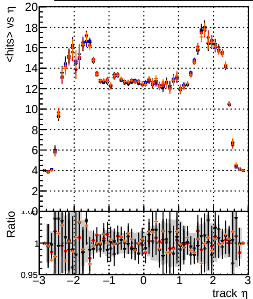
mean hit DQM_original_step2_ttbar-phase1-newgeom DQM_mkFit_step2_ttbar-phase1-newgeom DQM_angle_step2_ttbar-phase1-newgeom DQM_fast_step2_ttbar-phase1-newgeom
