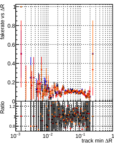
Fake rate vs \Delta R(\text{track, jet}) DOM original_step2_ttbar-phase1-newgeom DOM mkr-it_step2_ttbar-phase1-newgeom DOM angle_step2_ttbar-phase1-newgeom DOM fast_step2_ttbar-phase1-newgeom
