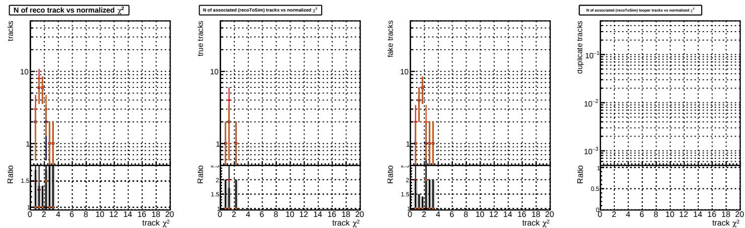
N of reco track vs. \chi^2
