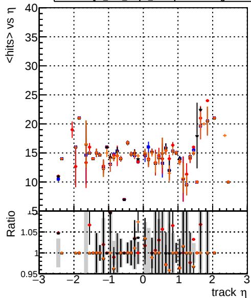
mean hit DQM_original_step2_ttbar-phase1-newgeom DQM_mkFit_step2_ttbar-phase1-newgeom DQM_angle_step2_ttbar-phase1-newgeom DQM_fast_step2_ttbar-phase1-newgeom
