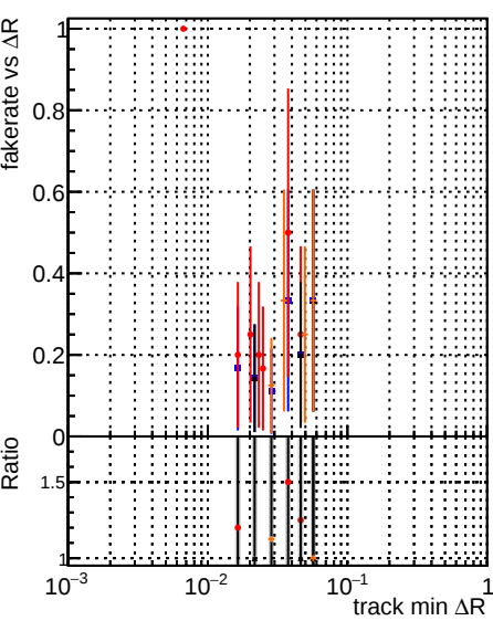
Fake rate vs \Delta R(\text{track, jet}) Legend: DOM original (blue) DOM mkt (red) DOM angle (black) DOM fast (orange) DOM original step2 ttbar-phase1-newgeom DOM mkt step2 ttbar-phase1-newgeom DOM angle step2 ttbar-phase1-newgeom DOM fast step2 ttbar-phase1-newgeom
