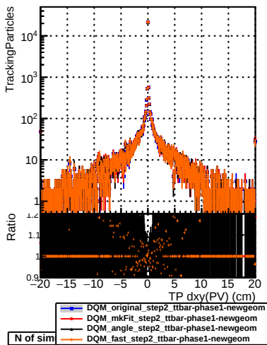
N of simulated tracks vs dxy(PV)
