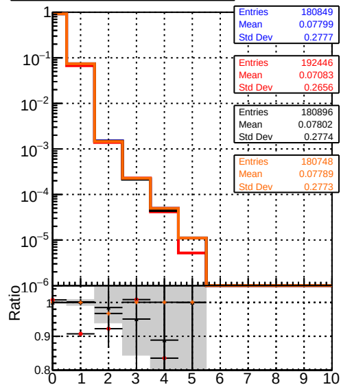
— DQM_original_step2_ttbar-phase1-newgeom — DQM_mkFit_step2_ttbar-phase1-newgeom — DQM_angle_step2_ttbar-phase1-newgeom — DQM_fast_step2_ttbar-phase1-newgeom
