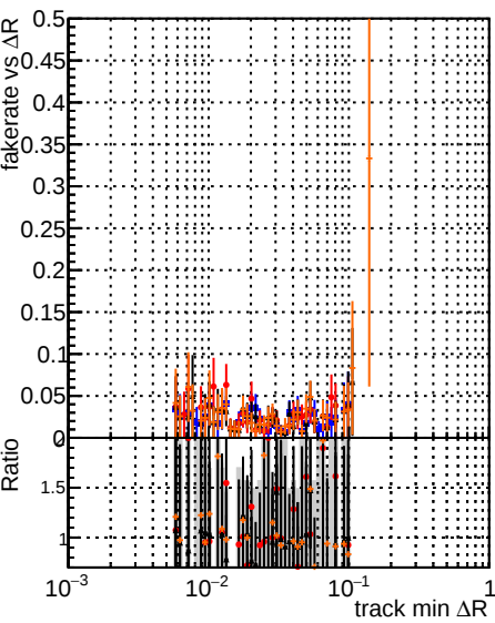
Fake rate vs \Delta R(\text{track}, \text{jet}) DOM original_step2_ttbare-phase1-newgeom DOM mkr_step2_ttbare-phase1-newgeom DOM angle_step2_ttbare-phase1-newgeom DOM fast_step2_ttbare-phase1-newgeom
