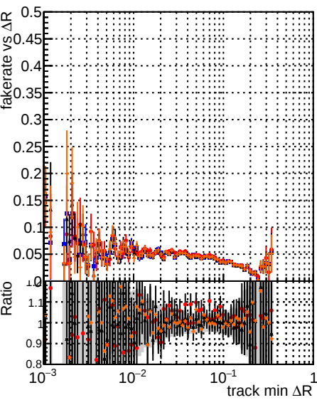
Fake rate vs \Delta R(\text{track}, \text{jet}) DOM original step2 tbar-phase1 newgeom DOM mkr-it step2 tbar-phase1 newgeom DOM angle step2 tbar-phase1 newgeom DOM fast step2 tbar-phase1 newgeom
