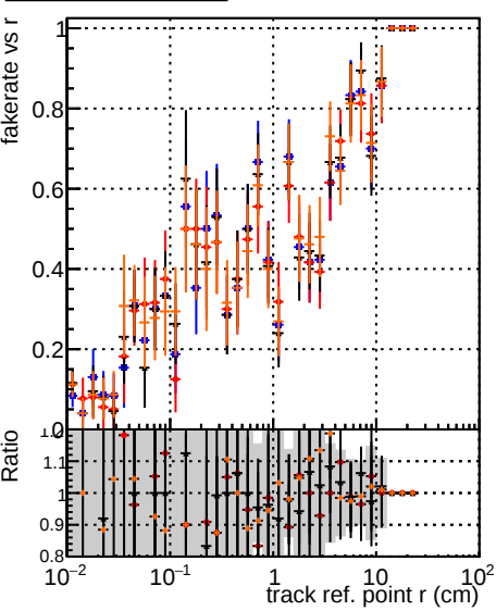
—■— DOM original_step2_ttbbar-phase1-newgeom —●— DOM mktit_step2_ttbbar-phase1-newgeom —▲— DOM angle_step2_ttbbar-phase1-newgeom —×— DOM fast_step2_ttbbar-phase1-newgeom
