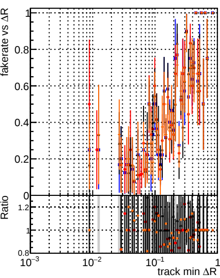
Fake rate vs \Delta R(\text{track, jet}) DOM original_step2_t1bar-phase1-newgeom DOM mkr-it_step2_t1bar-phase1-newgeom DOM angle_step2_t1bar-phase1-newgeom DOM fast_step2_t1bar-phase1-newgeom
