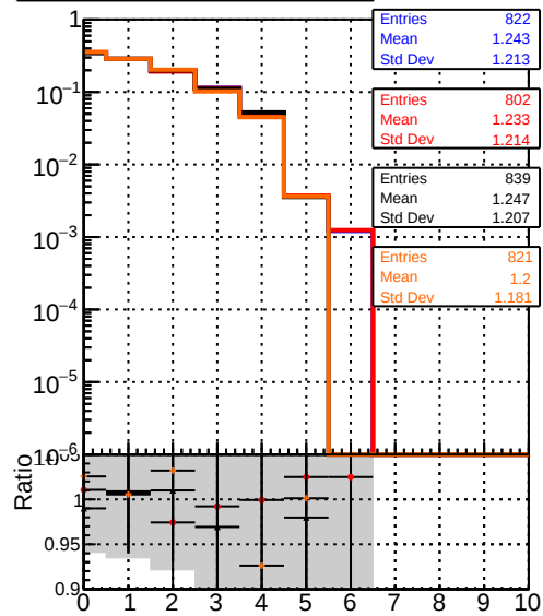
mean hits DQM_original_step2_ttbar-phase1-newgeom DQM_mkFit_step2_ttbar-phase1-newgeom DQM_angle_step2_ttbar-phase1-newgeom DQM_fast_step2_ttbar-phase1-newgeom
