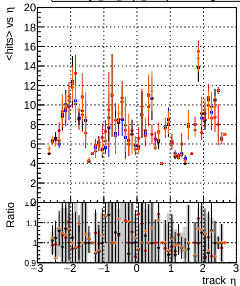
Legend: — DQM_original_step2_ttbar-phase1-newgeom — DQM_mkFit_step2_ttbar-phase1-newgeom — DQM_angle_step2_ttbar-phase1-newgeom — DQM_fast_step2_ttbar-phase1-newgeom
