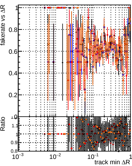
Fake rate vs \Delta R(\text{track, jet}) DOM original_step2_ttbart-phase1-newgeom DOM mkr-it_step2_ttbart-phase1-newgeom DOM angle_step2_ttbart-phase1-newgeom DOM fast_step2_ttbart-phase1-newgeom
