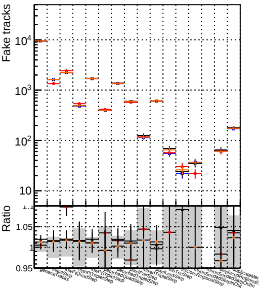
Number DQM_original_step2_ttbar-phase1-newgeom DQM_mkFit_step2_ttbar-phase1-newgeom DQM_angle_step2_ttbar-phase1-newgeom DQM_fast_step2_ttbar-phase1-newgeom
