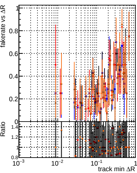
Fake rate vs \Delta R(\text{track, jet}) Legend: DOM original_step2_ttbare1-newgeom DOM mkr_step2_ttbare1-newgeom DOM angle_step2_ttbare1-newgeom DOM fast_step2_ttbare1-newgeom
