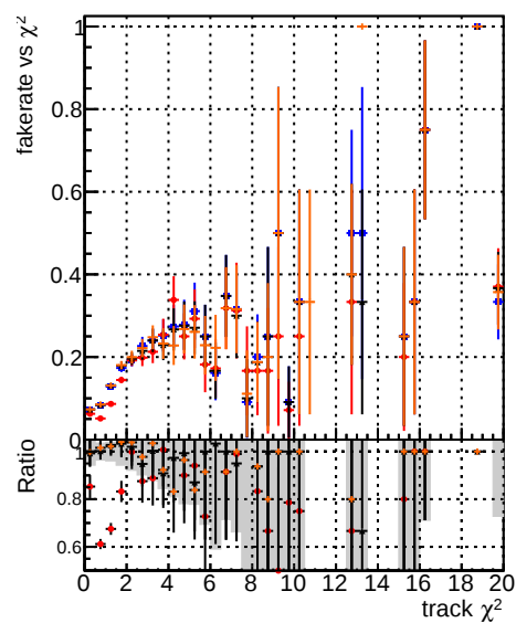
Fake rate vs. DQM original step2 ttbar phase1 newgeom DQM original step2 ttbar phase1 newgeom DQM original step2 ttbar phase1 newgeom DQM original step2 ttbar phase1 newgeom
