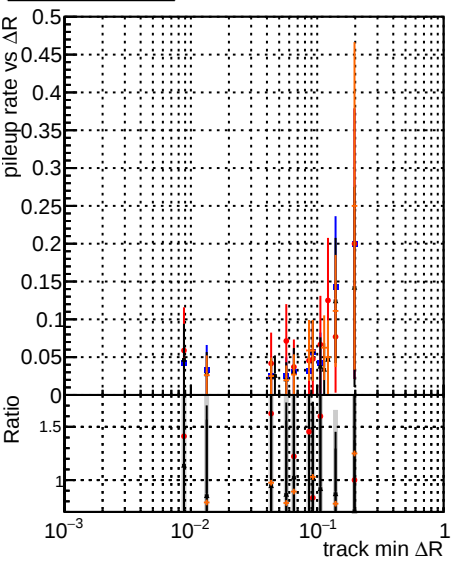
Legend: DOM original_step2_ttbar-phase1-newgeom DOM mkr-fit_step2_ttbar-phase1-newgeom DOM angle_step2_ttbar-phase1-newgeom DOM fast_step2_ttbar-phase1-newgeom
