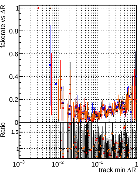
Fake rate vs \Delta R(\text{track, jet}) Legend: DQM original mkr-it angle fast
