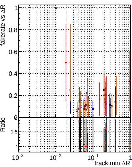
Fake rate vs \Delta R(\text{track}, \text{jet}) DOM original step2 ttbar-phase1-newgeom DOM mkr step2 ttbar-phase1-newgeom DOM angle step2 ttbar-phase1-newgeom DOM fast step2 ttbar-phase1-newgeom
