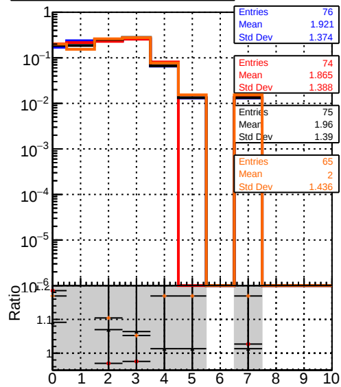
mean hit DQM_original_step2_ttbbar-phase1-newgeom DQM_mkFit_step2_ttbbar-phase1-newgeom DQM_angle_step2_ttbbar-phase1-newgeom DQM_fast_step2_ttbbar-phase1-newgeom
