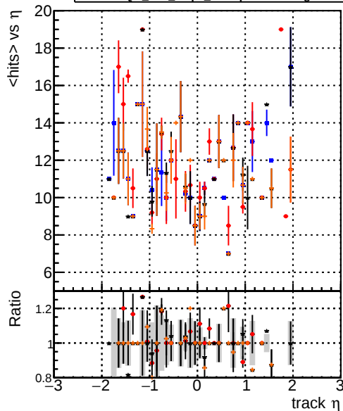
mean hit DQM_original_step2_ttbbar-phase1-newgeom DQM_mkFit_step2_ttbbar-phase1-newgeom DQM_angle_step2_ttbbar-phase1-newgeom DQM_fast_step2_ttbbar-phase1-newgeom
