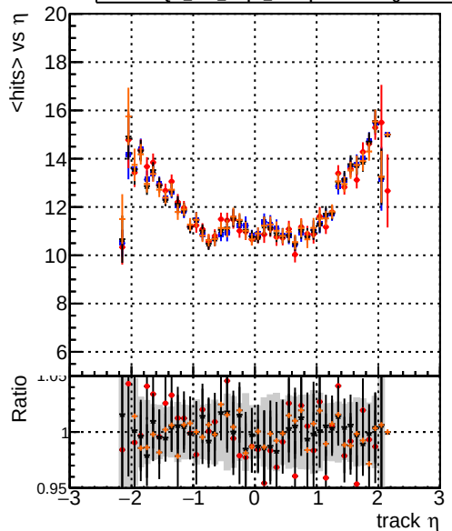
mean hit DOM_original_step2_ttbar-phase1-newgeom DOM_mkFit_step2_ttbar-phase1-newgeom DOM_angle_step2_ttbar-phase1-newgeom DOM_fast_step2_ttbar-phase1-newgeom
