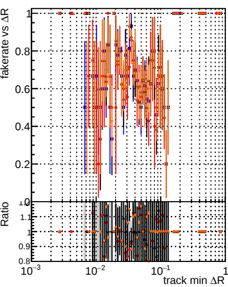
Fake rate vs \Delta R(\text{track, jet}) Legend: DOM original (blue) DOM mkr-it (red) DOM angle (black) DOM fast (orange)
