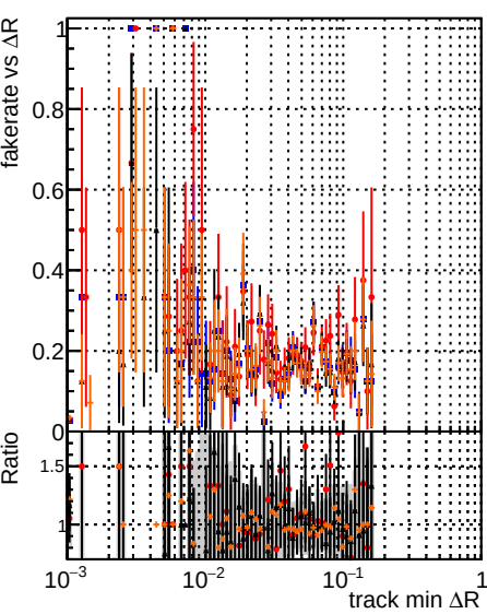
Legend: original (blue), step2 (red), ttbar-phase1 (black), newgeom (orange). Fake rate vs \Delta R (track, jet)
