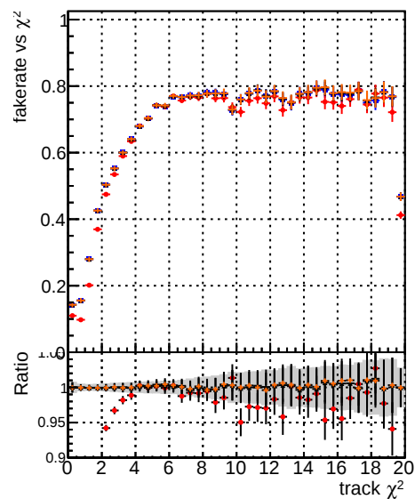
Fake rate vs. \chi^2 DOM original_step2_tbar_phase1_newgeom DOM original_step2_tbar_phase1_newgeom DOM original_step2_tbar_phase1_newgeom DOM original_step2_tbar_phase1_newgeom
