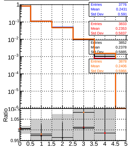
mean hit — DQM_original_step2_ttbar-phase1-newgeom — DQM_mkFit_step2_ttbar-phase1-newgeom — DQM_angle_step2_ttbar-phase1-newgeom — DQM_fast_step2_ttbar-phase1-newgeom
