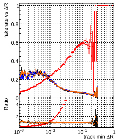
DQM original step2 ttbar-phase1-newgeom DQM mkr-it step2 ttbar-phase1-newgeom DQM angle step2 ttbar-phase1-newgeom DQM fast step2 ttbar-phase1-newgeom
