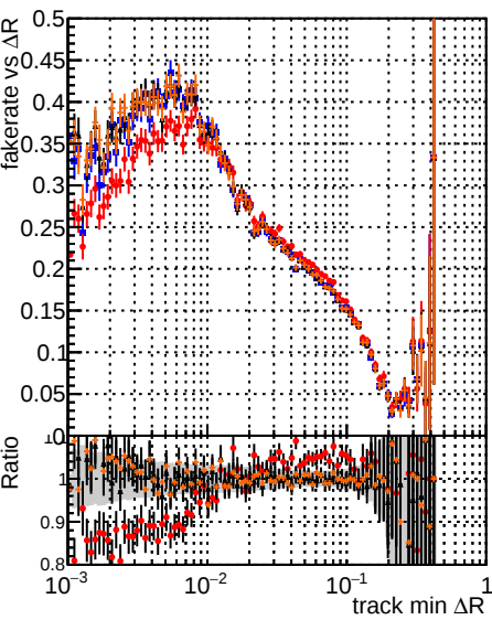
Fake rate vs \Delta R(\text{track, jet}) Legend: DOM original_step2_ttbbar-phase1-newgeom (blue squares) DOM mkr-it_step2_ttbbar-phase1-newgeom (red circles) DOM angle_step2_ttbbar-phase1-newgeom (black triangles) DOM fast_step2_ttbbar-phase1-newgeom (orange diamonds)
