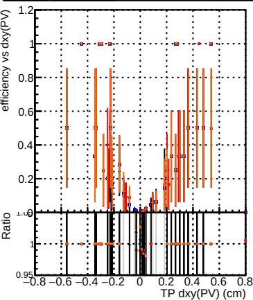
Efficiency vs Dxy(PV) Legend: DQM_original_step2_ttbar-phase1-newgeom DQM_mkFit_step2_ttbar-phase1-newgeom DQM_angle_step2_ttbar-phase1-newgeom DQM_fast_step2_ttbar-phase1-newgeom
