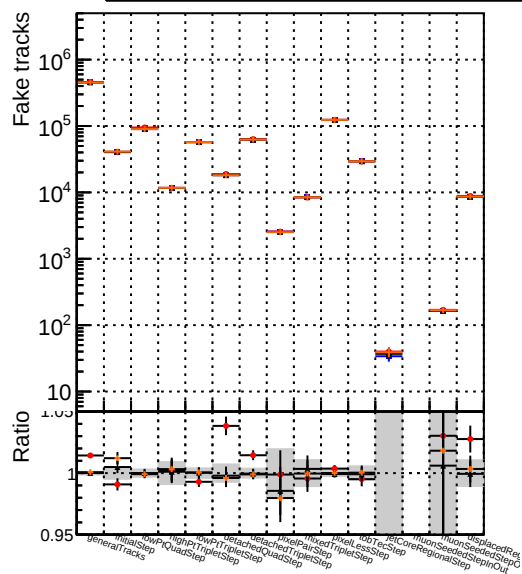
Number —●— DQM_angle_step2_ttbar-phase1-newgeom —▲— DQM_angle_step2_ttbar-phase1-newgeom —+— DQM_fast_step2_ttbar-phase1-newgeom
