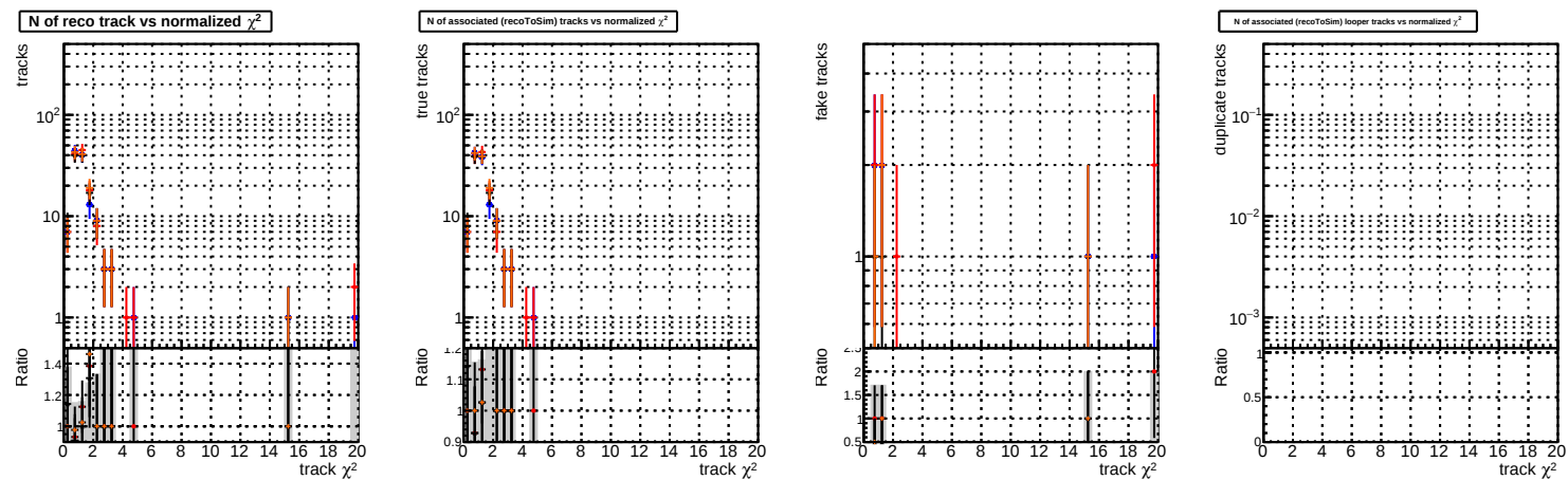
N of reco track vs. \chi^2 Legend: Blue line with circles: BDM original step2 tbar phase1 newgeom Orange line with circles: BDM original step2 tbar phase1 newgeom Red line with circles: BDM original step2 tbar phase1 newgeom Black line with circles: BDM fast step2 tbar phase1 newgeom
