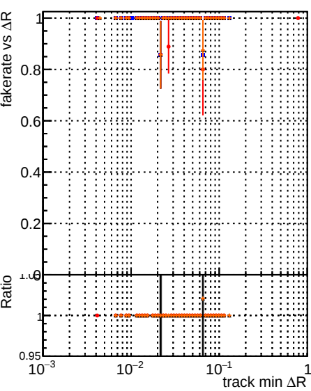
Fake rate vs \Delta R(\text{track, jet}) Legend: DOM original (blue line with dots) DOM mkt (red line with dots) DOM angle (black line with dots) DOM fast (orange line with dots) DOM original step2 ttbar-phase1-newgeom DOM mkt step2 ttbar-phase1-newgeom DOM angle step2 ttbar-phase1-newgeom DOM fast step2 ttbar-phase1-newgeom
