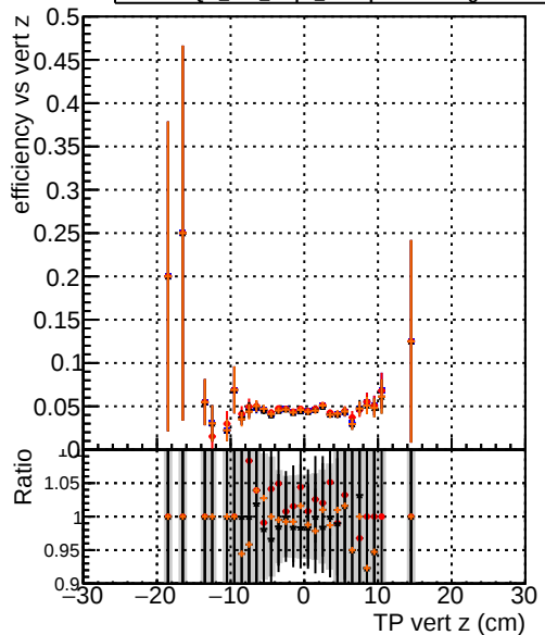
Efficiency vs vert z —●— DQM_original_step2_ttbar-phase1-newgeom —●— DQM_mkFit_step2_ttbar-phase1-newgeom —●— DQM_angle_step2_ttbar-phase1-newgeom —●— DQM_fast_step2_ttbar-phase1-newgeom
