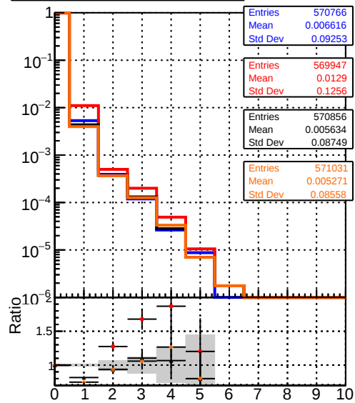
mean hit Legend: Blue line: DQM_original_step2_ttbar-phase1-newgeom Red line: DQM_mkFit_step2_ttbar-phase1-newgeom Black line: DQM_angle_step2_ttbar-phase1-newgeom Orange line: DQM_fast_step2_ttbar-phase1-newgeom
