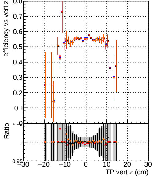
Efficiency vs. TP vert z — DQM_original_step2_ttbar-phase1-newgeom — DQM_mkFit_step2_ttbar-phase1-newgeom — DQM_angle_step2_ttbar-phase1-newgeom — DQM_fast_step2_ttbar-phase1-newgeom
