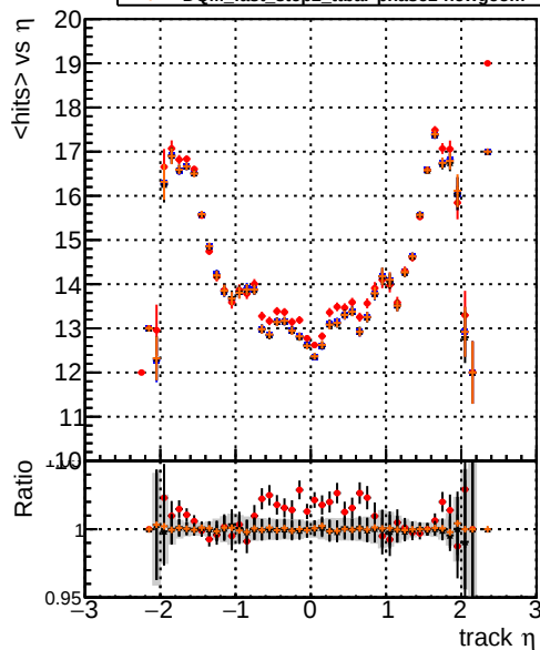
mean hits vs \eta Legend: Blue line: DQM_original_step2_ttbar-phase1-newgeom Red line: DQM_mkFit_step2_ttbar-phase1-newgeom Black line: DQM_angle_step2_ttbar-phase1-newgeom Orange line: DQM_fast_step2_ttbar-phase1-newgeom
