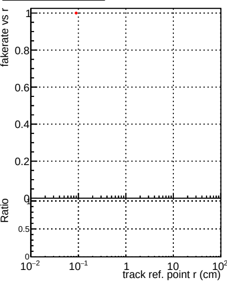
DOM original step2 pt1to20 eta2p5to4p0 DOM mkfit step2 pt1to20 eta2p5to4p0 DOM angle step2 pt1to20 eta2p5to4p0 DOM fast step2 pt1to20 eta2p5to4p0
