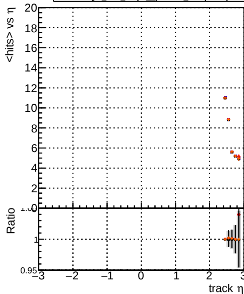
mean hit — DQM_original_step2_pt1to20_eta2p5to4p0 — DQM_mkFit_step2_pt1to20_eta2p5to4p0 — DQM_angle_step2_pt1to20_eta2p5to4p0 — DQM_fast_step2_pt1to20_eta2p5to4p0
