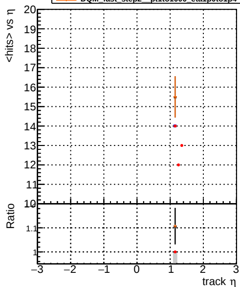
mean hit DQM_original_step2_pt10to1000_eta1p0to1p4 DQM_mkFit_step2_pt10to1000_eta1p0to1p4 DQM_angle_step2_pt10to1000_eta1p0to1p4 DQM_fast_step2_pt10to1000_eta1p0to1p4
