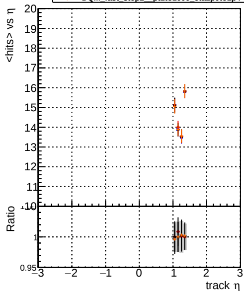
mean hit — DQM_original_step2_pt1to1000_eta1p0to1p4 — DQM_mkFit_step2_pt1to1000_eta1p0to1p4 — DQM_angle_step2_pt1to1000_eta1p0to1p4 — DQM_fast_step2_pt1to1000_eta1p0to1p4
