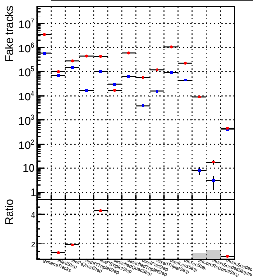
Number —●— DOM CKF TTbar
