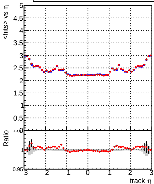
mean hits vs \eta Legend: DQM_TTbarTEST (blue line), DQM_CKF_TTbar (red line)
