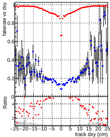
—●— DQM_TTbarTEST —●— DQM_CKF_TTbar
