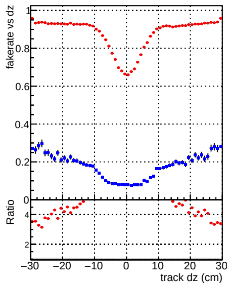
—●— DQM_TTbarTEST —●— DQM_CKF_TTbar
