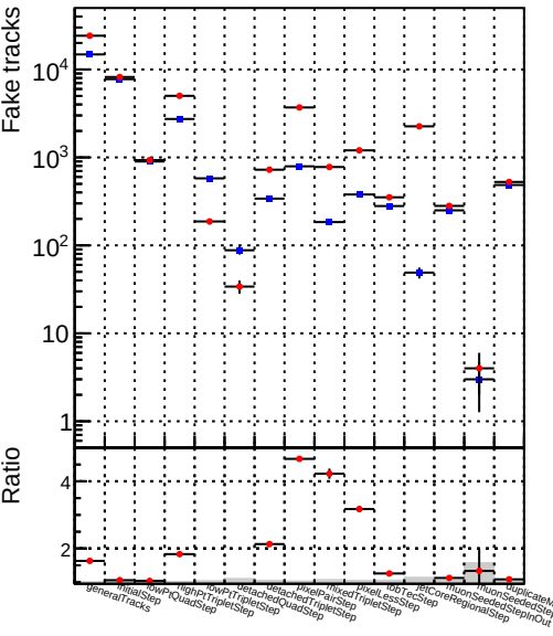
Number —●— DQM_CKF_TTbar
