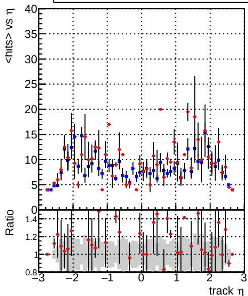
mean hit — DQM_TTbarTEST — DQM_CKF_TTbar
